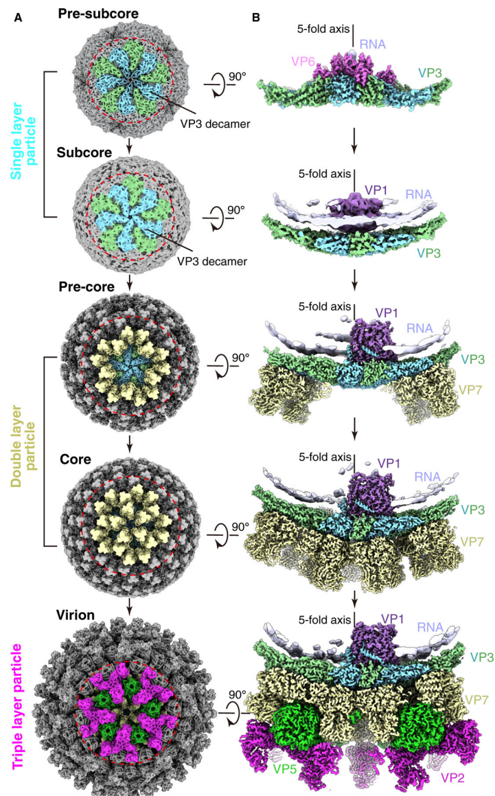
Figure 2. High-resolution structures of BTV assembly intermediates resolved by cryo-EM (A) Cryo-EM maps from icosahedral reconstruction of BTV assembly intermediates. Among the eight states shown in Figure S2, only five contain RNA and are shown here. For each viral particle, structures around one of the 12 vertices are colored. The red circle demarcates the area for sub-particle reconstruction. (B) Corresponding vertex reconstructions by sub-particle boxed out from the BTV assembly intermediates in (A). Densities segmented out for different protein and RNA molecules are colored differently, as labeled. See also workflow and additional assembly states in Figure S2.
