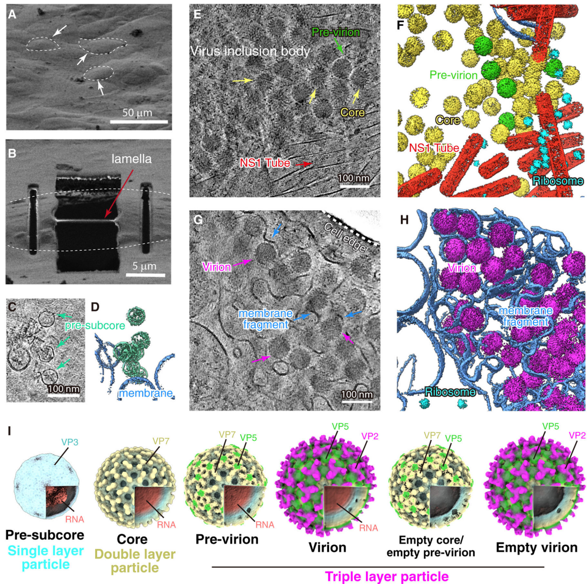
Figure 1. BTV assembly intermediates in the host cytoplasm captured by cellular cryo-ET (A) Scanning electron microscope (SEM) image of infected cells on EM grid prior to cryo-FIB milling. Example cells are outlined by dashed lines and indicated by arrows. (B) SEM image of a cell after FIB milling. Outline of the cell is indicated by dashed lines. (C and D) A slice image (C) and corresponding 3D segmentation (D) from the cryo-ET reconstruction, showing the assembled pre-subcore. (E and F) A slice image (E) and corresponding 3D segmentation (F) from a cryo-ET reconstruction, showing the BTV assembly intermediates within a virus inclusion body. (G and H) A slice image (G) and corresponding 3D segmentation (H) of cryo-ET reconstruction, showing that virus egress is associated with membranes at the cell periphery. (I) Six states of BTV assembly captured by cellular tomography. See also Figure S1 and Video S1 related to (E) and (F) and Video S2 related to (G) and (H).
