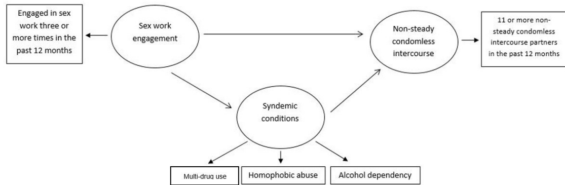
Figure 1. SEM model to be tested
