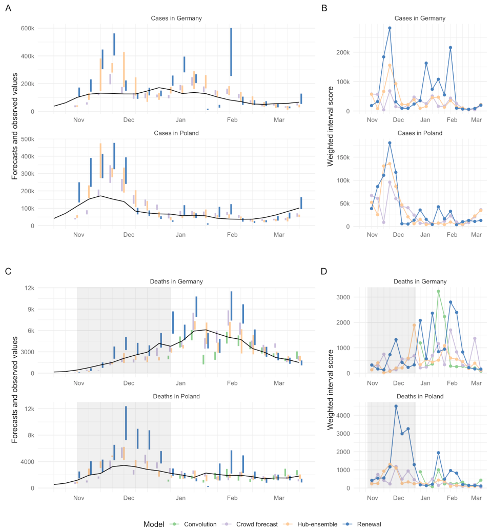
Fig S10. A, C: Visualisation of 50% prediction intervals of three week ahead forecasts against the reported values. Forecasts that were not scored (because there was no complete set of death forecasts available) are greyed out. B, D: Visualisation of corresponding WIS.
