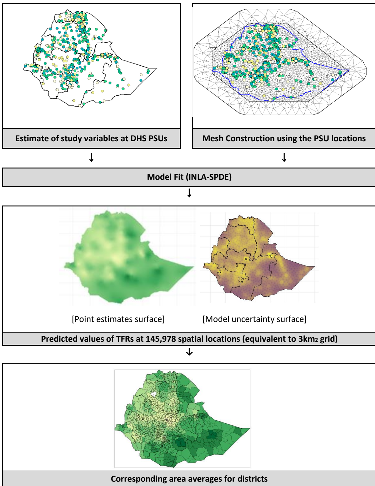
Figure 3.5. Geostatistical modelled prediction process
