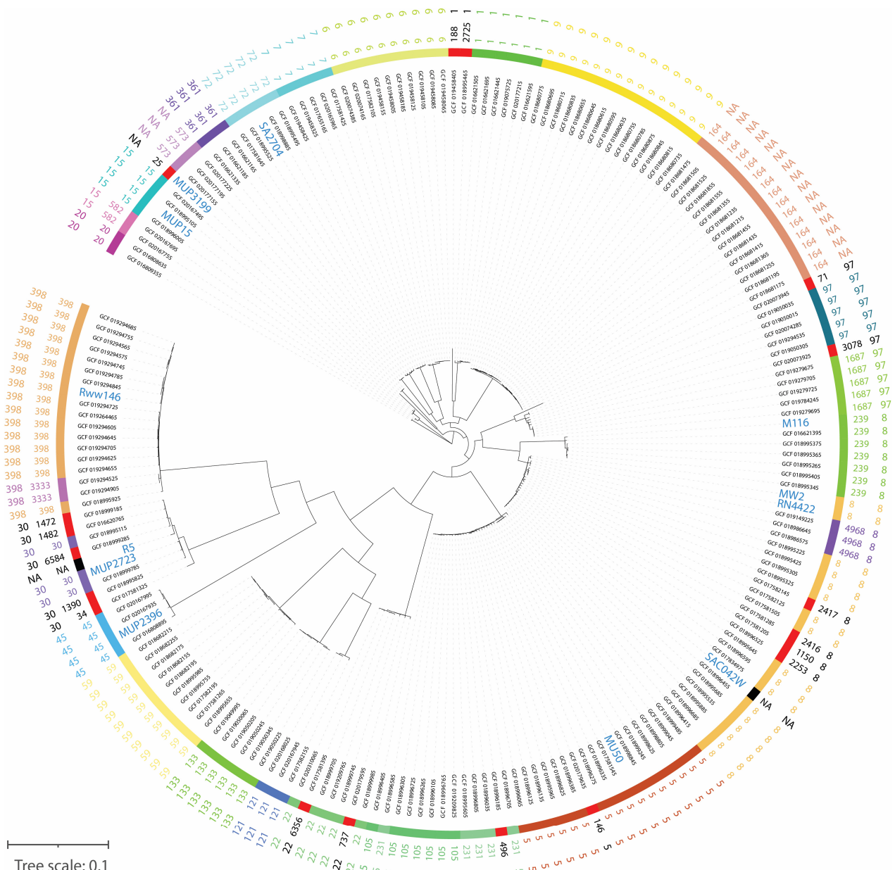
Figure 1. Circular visualization of the genomes of S. aureus strains in our panel compared to 205 S. aureus strains representing global genetic diversity. The maximum-likelihood tree in the figure describes the core SNP differences. From the inner to the outer circle, the first circle represents public genomes of S. aureus including the genomes from this study marked in blue and larger font, the second and third circles represents sequence type (ST) characterization visualized by color and text and the fourth circle represents CC information. Genomes without an ST and CC identification were symbolized with NA (Non-Available).
