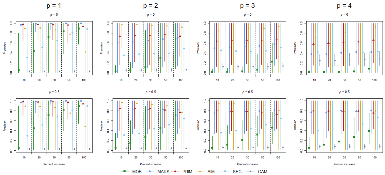
Figure S2: Mean and 95% confidence interval of precision for each simulation scenario.
