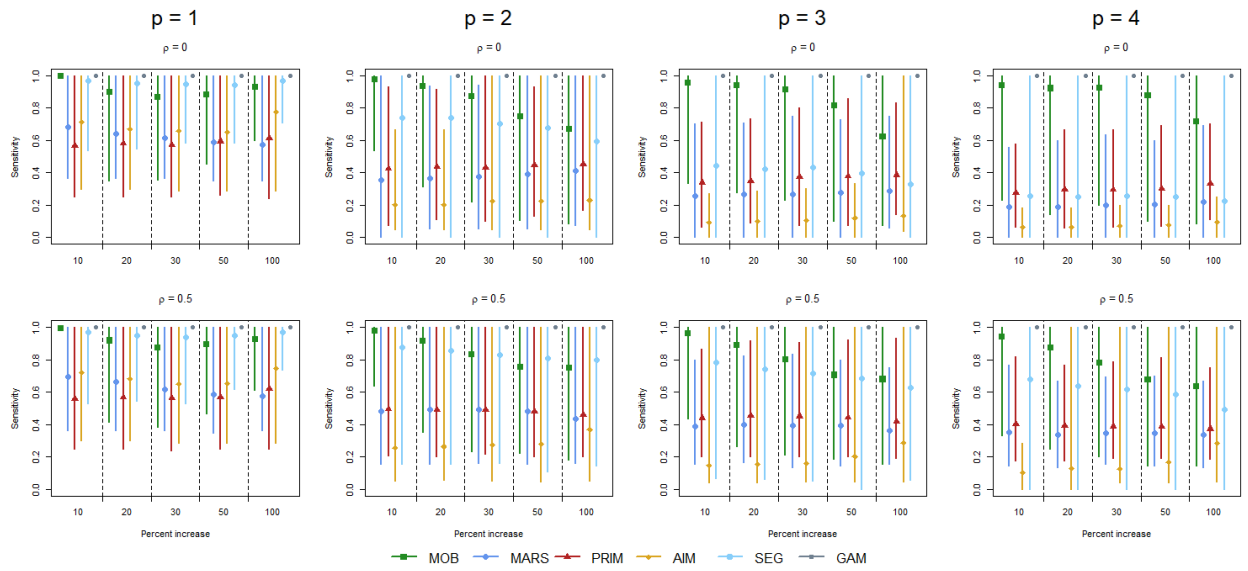
Figure S1: Mean and 95% confidence interval of sensitivity for each simulation scenario.
