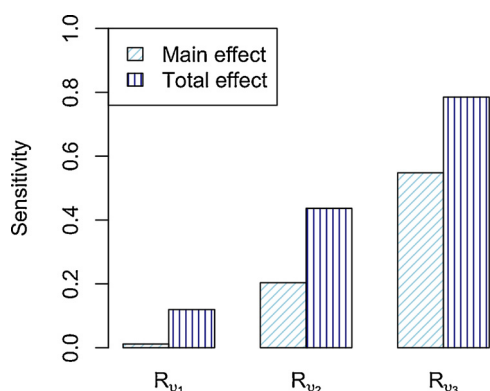
Fig. 3. Main and total effect for the different components of R_0 > 1 .
