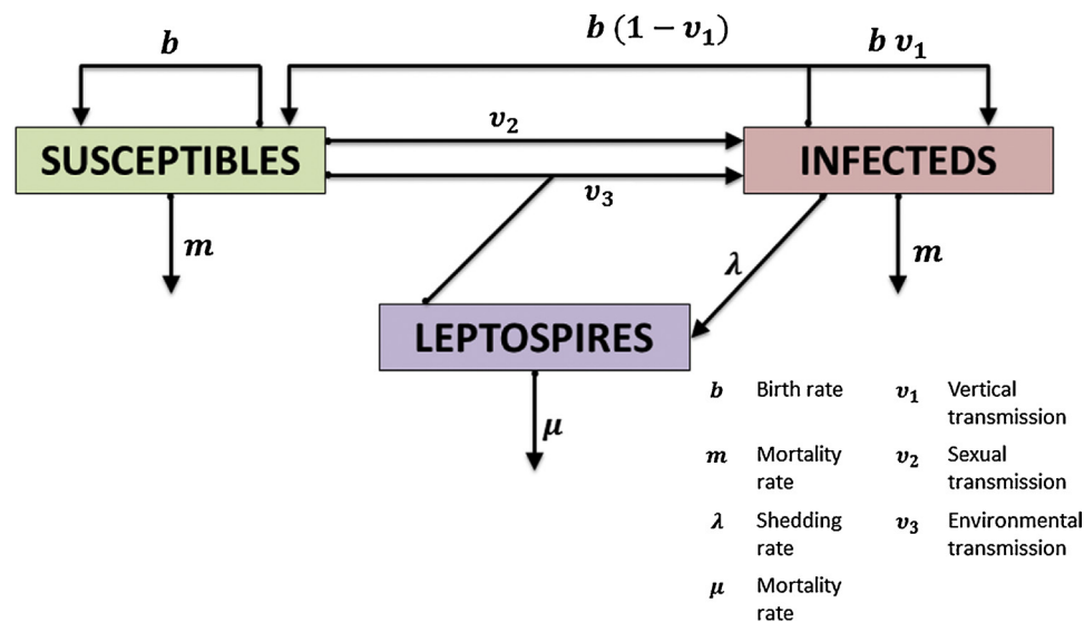
Fig. 1. Flow diagram of leptospire dynamics in rats.
