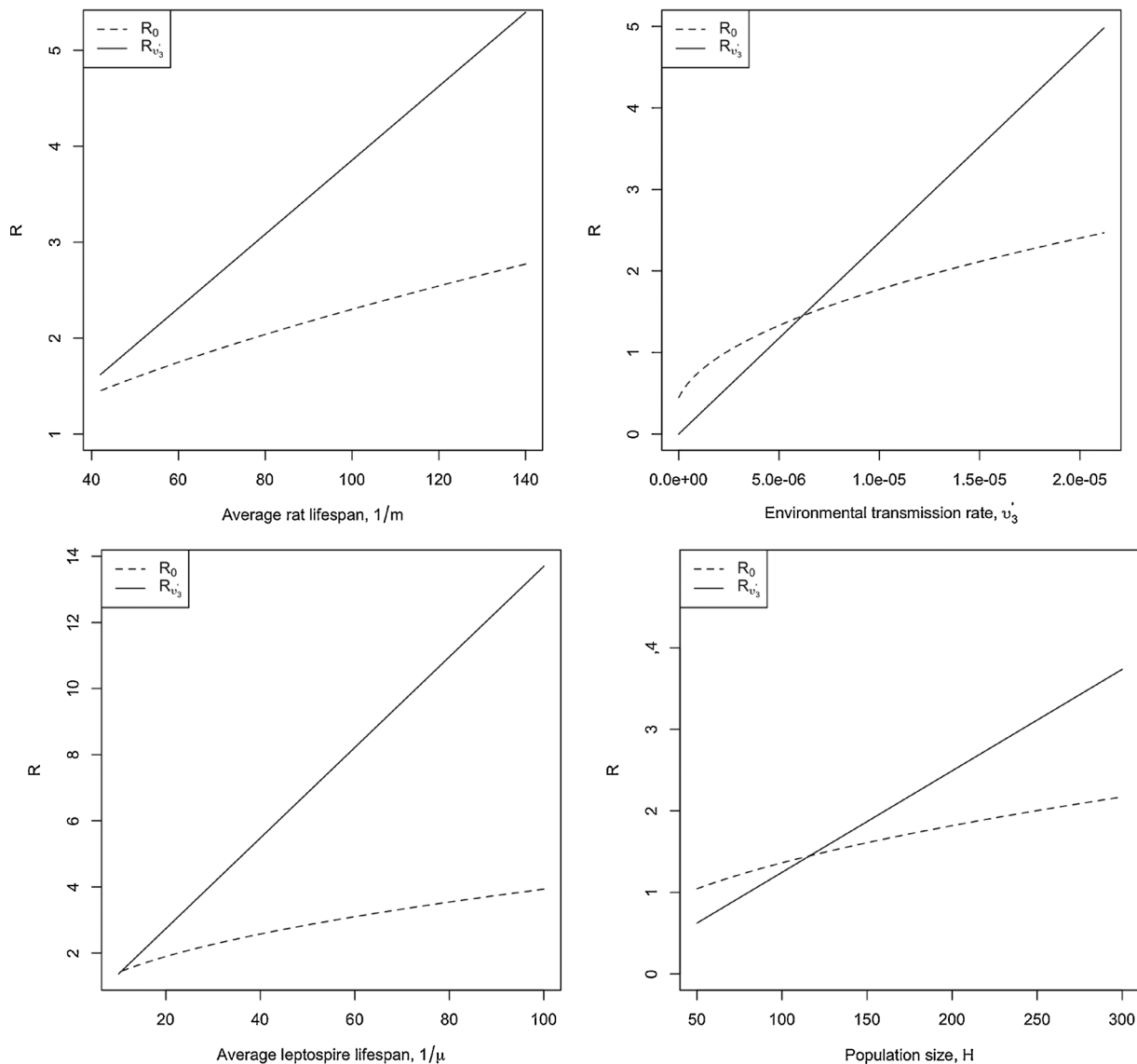
Fig. 4. Changes in the basic reproduction number R_0 (dashed line) and the basic reproduction number for environmental transmission only R_{v_3'} (solid line) and with respect to changes in mortality rate m , environmental transmission rate v_3' , leptospire mortality rate \mu and population size H .
