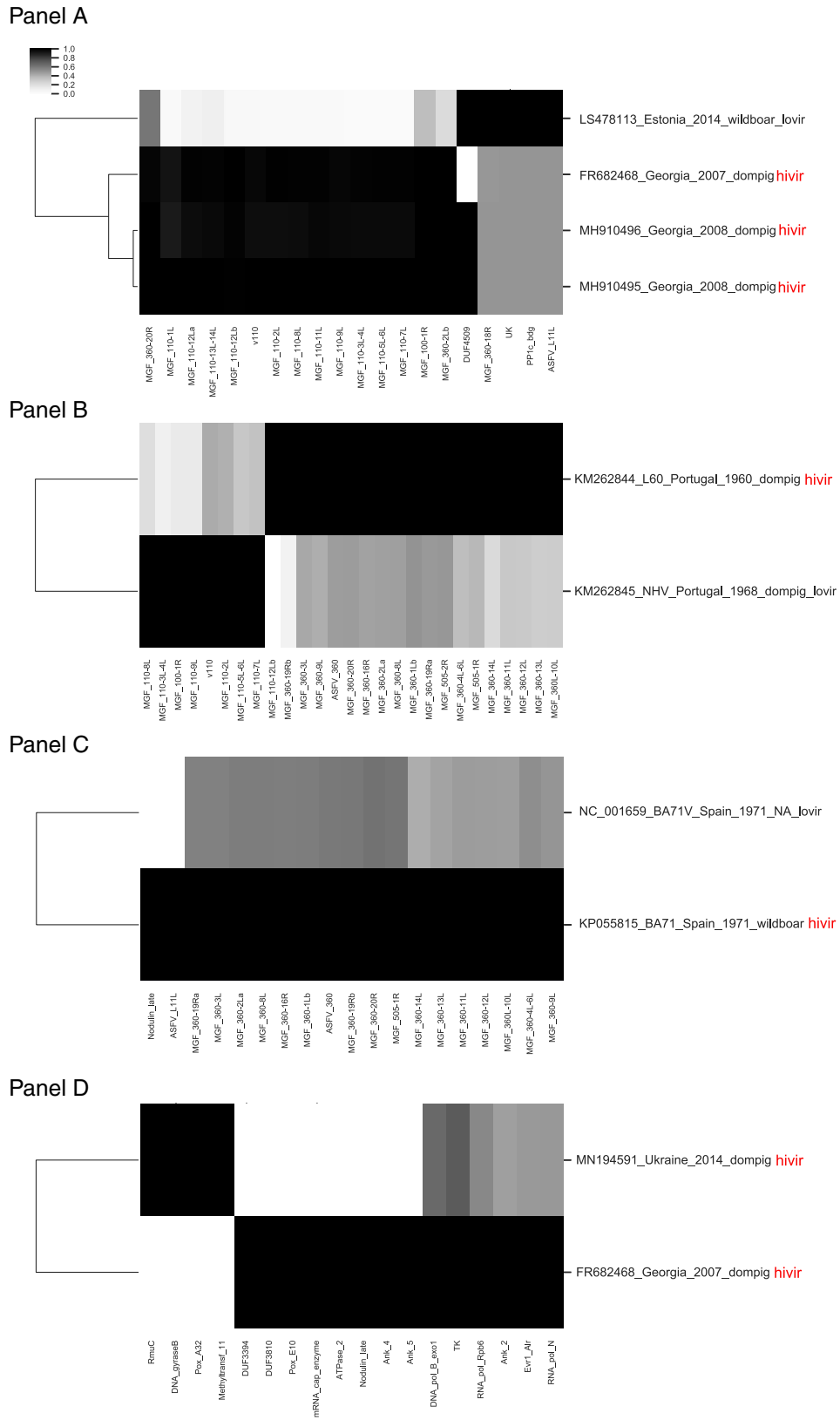
Figure 5. Differences in domains between paired ASFV strains. For each panel, the indicated genomes were examined for Pfam and MGF domain content, the bit-scores for all domains identified with domain i -Evalue <0.0001 were collected for each domain, and a matrix was prepared and subjected to hierarchical clustering (see Section 2) based on domain whose normalized values showed \geq 0.03 variance. Genome IDs (Y axis) include GenBank accession number, strain_name, country, date, host, and virulence (lovir = low-reported virulence, hivir = high-reported virulence).
