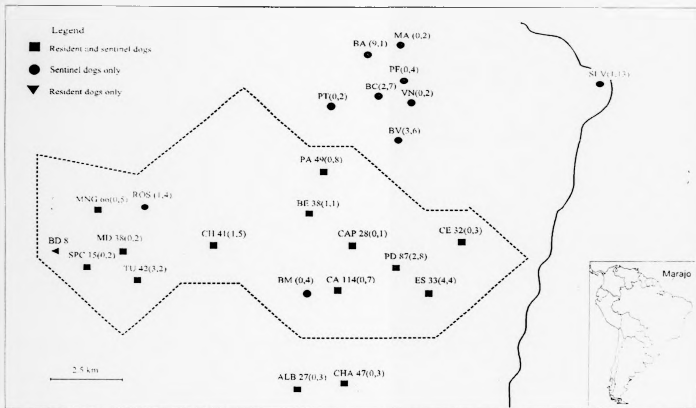
Figure 2.1 The distribution of study villages (symbols) in Marajó, Brazil (inset) showing the number of resident dogs per village. The numbers of local and Belem sentinel dogs, respectively, are shown in brackets (-----) demarks the area in which study foxes were trapped
