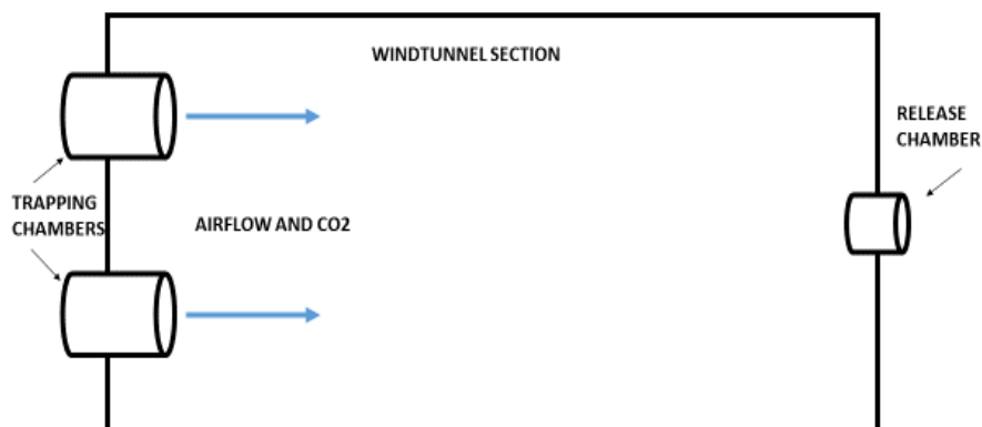
Figure 2-3. The dual-choice windtunnel olfactometer used to test measure behavioural responses of An. stephensi to odour stimuli.
