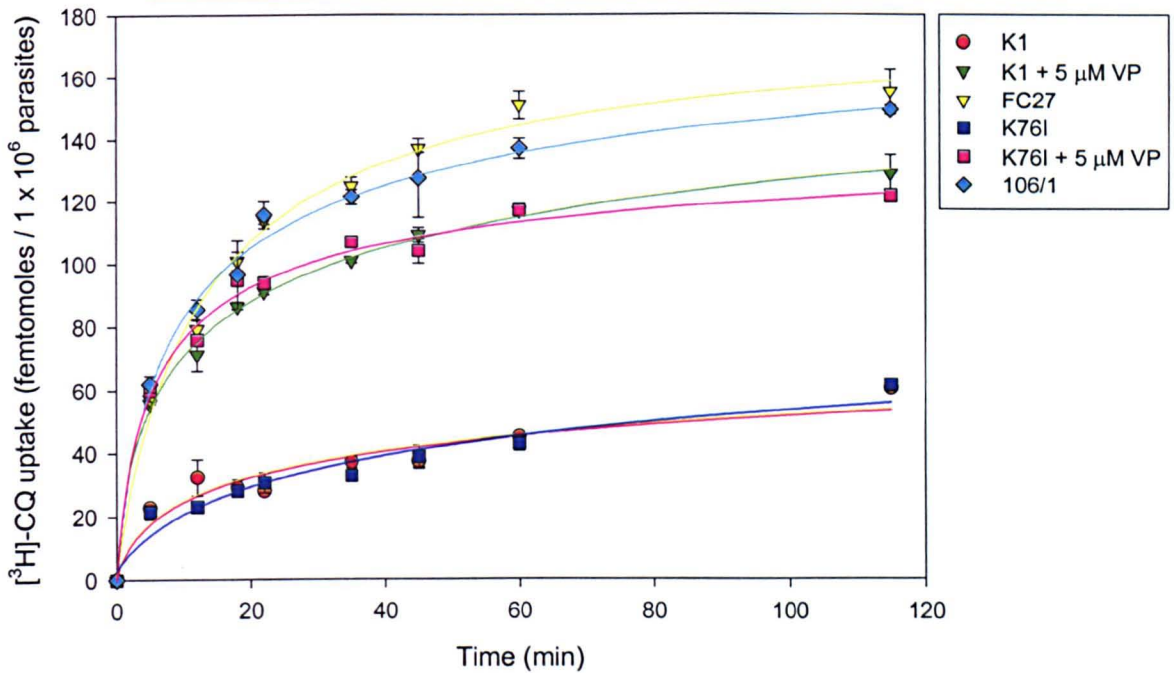
Figure 5.8: Time course of 5 nM [ 3 H]-CQ uptake by RBC infected with K1, FC27, K76I and 106/1 parasite lines demonstrating the role of pfcr1 mutations in CQ uptake. §
