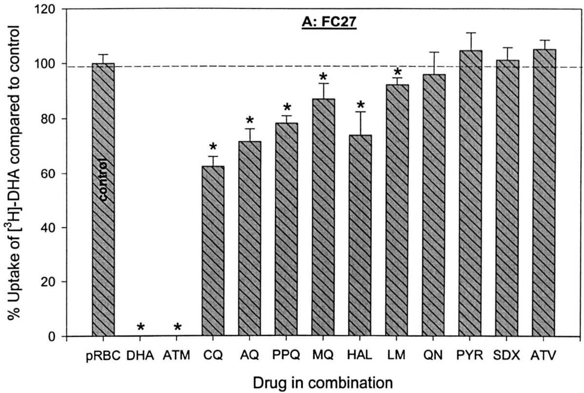
Figure 5.4: Effects of antimalarials at 3 \mu\text{M} on the uptake of 3 nM [ ^3\text{H} ]-DHA after 90 min in RBC infected with P. falciparum . ‡
