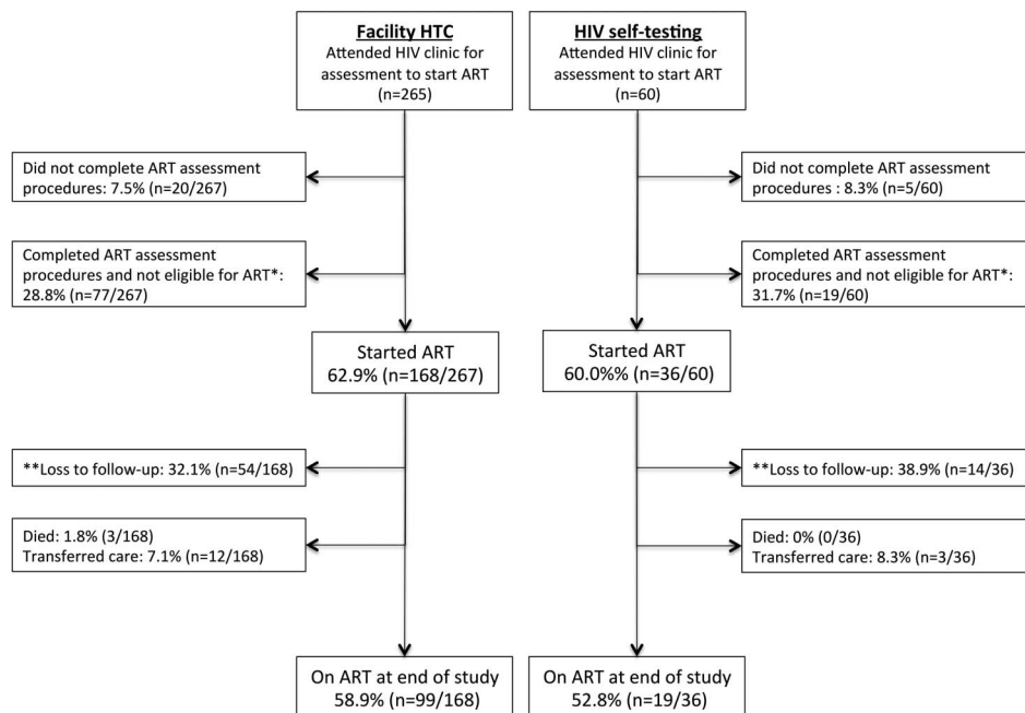
FIGURE 1. Participant recruitment and follow-up. *Malawi national ART eligibility criteria during study period: CD4 count <350 cells/mm 3 ; WHO stage 3 or 4; breastfeeding; or pregnant. **Loss to follow-up from this health economic study.
