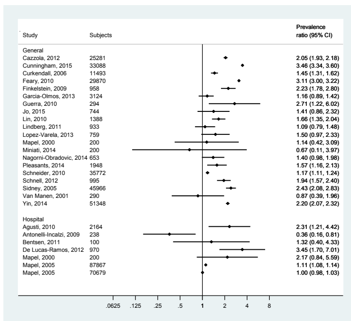
Figure A4.1 Forest plot showing estimates of the prevalence ratio (PR) for stroke comparing people with and without COPD, grouped according to population characteristics
