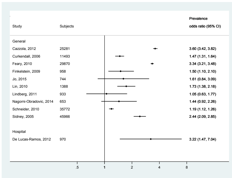
Figure A4.3 Forest plot showing estimates of the prevalence odds ratio (POR) for stroke comparing people with and without COPD, grouped according to population characteristics
