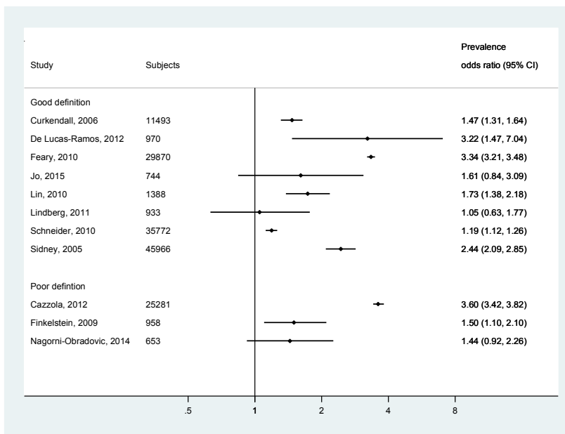
Figure A4.4 Forest plot showing estimates of the prevalence odds ratio (POR) for stroke comparing people with and without COPD, grouped according to quality of COPD case definition
