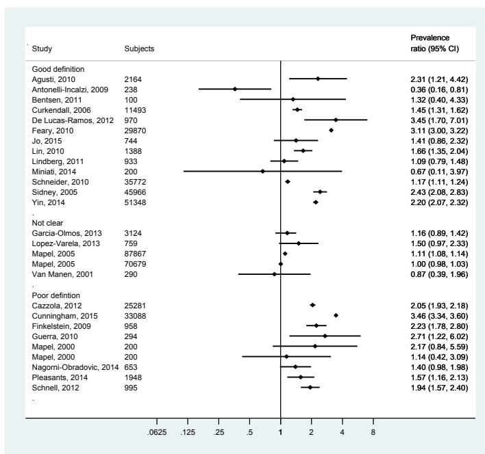
Figure A4.2 Forest plot showing estimates of the prevalence ratio (PR) for stroke comparing people with and without COPD, grouped according to quality of COPD case definition
