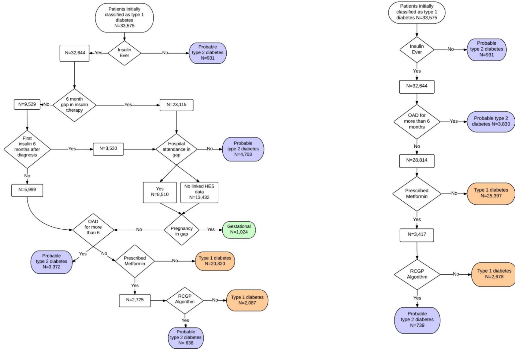
Figure 7.3 Detecting errors in type 1 diabetes: Results for full and simplified algorithms
