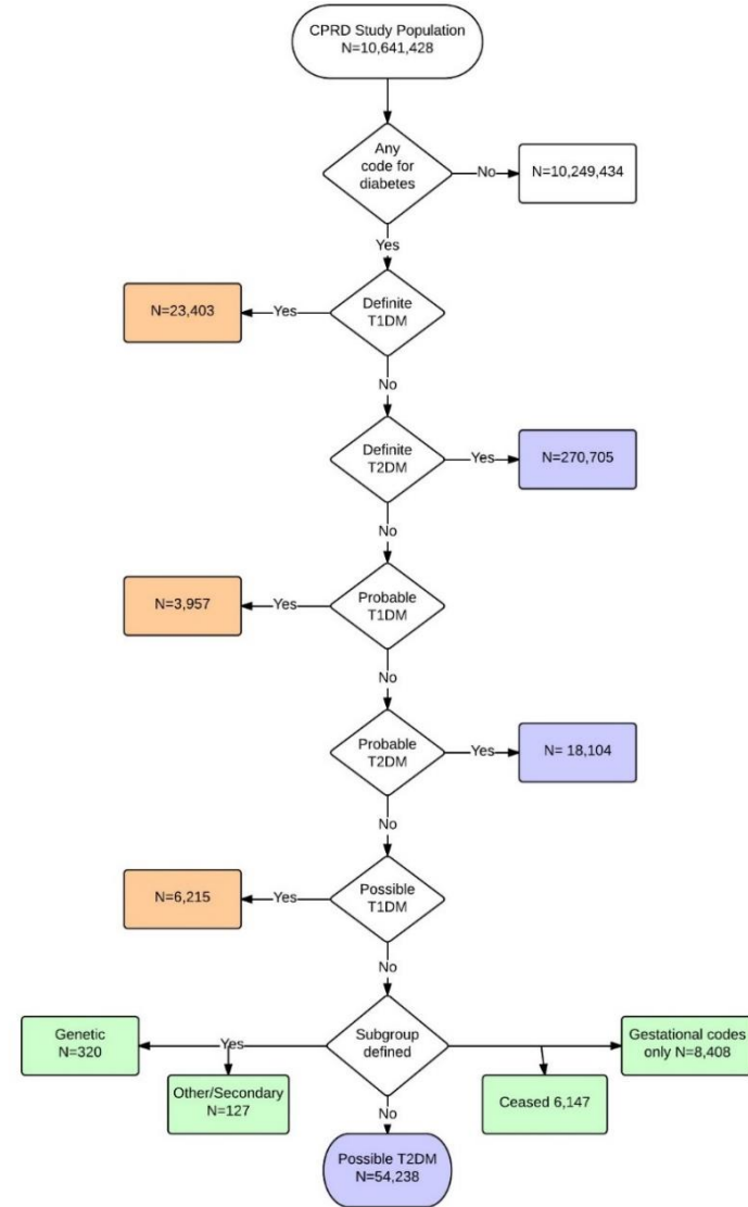
Figure 7.2 Initial Sort and Classification Results
