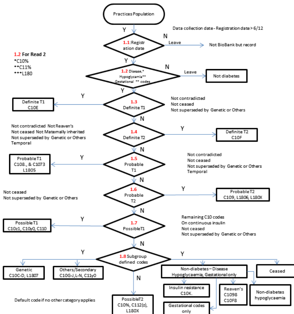
Figure 6.1 Flowchart 1: Initial Sort and Classification of diabetes type
