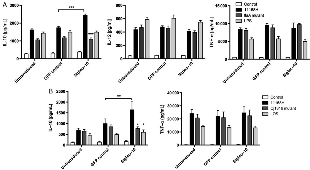
Figure 5. Siglec-10 receptor overexpression promotes IL-10 expression in response to Campylobacter jejuni flagella. A, Untransduced, GFP control, and Siglec-10 transduced PMA-differentiated THP-1 cells were infected with 11168H WT and flaA isogenic mutant (MOI 100) or LPS (100 ng/mL) for 24 hours. B, Untransduced, GFP control and Siglec-10 transduced RAW264.7 were infected with 11168H WT and Cj1316 isogenic mutant (MOI 100) or purified C. jejuni 11168H LOS (100 ng/mL) for 24 hours. IL-10, IL-12 and TNF \alpha protein levels were assessed by ELISA. Bars depict data from 4 independent experiments \pm SEM. Friedman statistical analysis was performed on data sets. * P < .05 ; ** P < .01 ; *** P < .001 . Abbreviations: ELISA, enzyme-linked immunosorbent assay; IL, interleukin; MOI, multiplicity of infection; SEM, standard error of the mean; TNF \alpha , tumor necrosis factor \alpha ; WT, wild-type.
