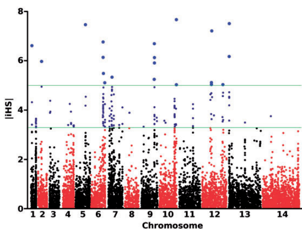
Fig. 4. Genome-wide scan of standardized |iHS| for P. falciparum SNPs with minor allele frequency of at least 5% in N'Zerekore (Guinea, sequence analysis of 100 clinical isolates). Individual chromosomes are identified by alternate black and red coloring of their SNPs, with high scoring SNPs highlighted ( |iHS| > 3.29 [top 1% of expected distribution] in dark blue and > 5 with enlarged light blue symbols), indicating loci most likely to have been under recent positive directional selection.
