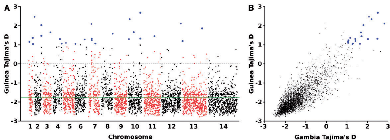
Fig. 3. Genome-wide distribution of Tajima's D values summarizing the allele frequency spectra for P. falciparum genes with three or more SNPs. (A) Tajima's D values for each of 4,012 P. falciparum genes with three or more SNPs in Guinea (N'Zerekore population sample of 100 isolate sequences). Individual chromosomes are identified by the alternate black and red coloring with genes plotted as individual points based on their position within each chromosome. Genes with Tajima's D values > 1 are highlighted with enlarged blue symbols. Detailed data for each of the genes are given in supplementary table S3, Supplementary Material online. (B) Correlation between Tajima's D scores for the Guinea (N'Zerekore) population and a previously sampled population from The Gambia (Greater Banjul area), analyzing 3,316 genes that had three or more SNPs in each of the populations. Genes with a Tajima's D value of > 1 in both populations are highlighted with enlarged blue symbols (and identified in table 1 ).
