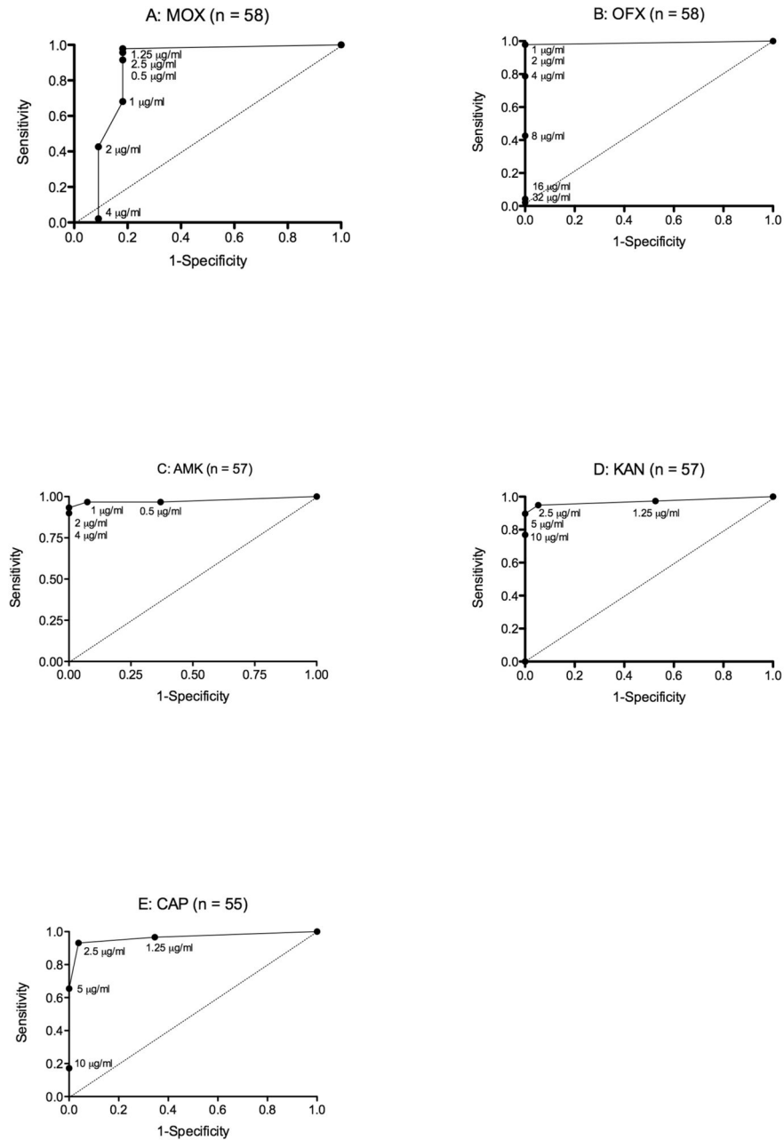
Figure 1. ROC curves for (A) MOX, (B) OFX, (C) AMK, (D) KAN, (E) CAP. Drug concentrations that reach furthest to the top left corner represent those with highest sensitivity and specificity, and these were selected as the candidate breakpoints for the MODS second-line DST assay
