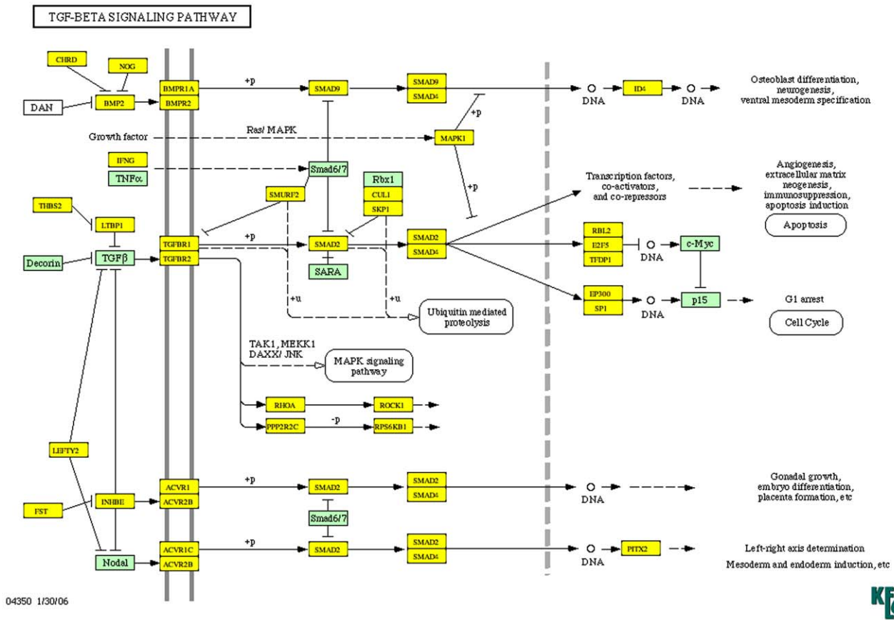
Figure 4. TGF-β signaling pathway. Genes highlighted in yellow are predicted targets of miR differentially regulated in N v TSI (35 miR) ( FC > 3 , p < 0.05 ). Genes highlighted in green are not predicted targets. doi:10.1371/journal.pntd.0002117.g004
