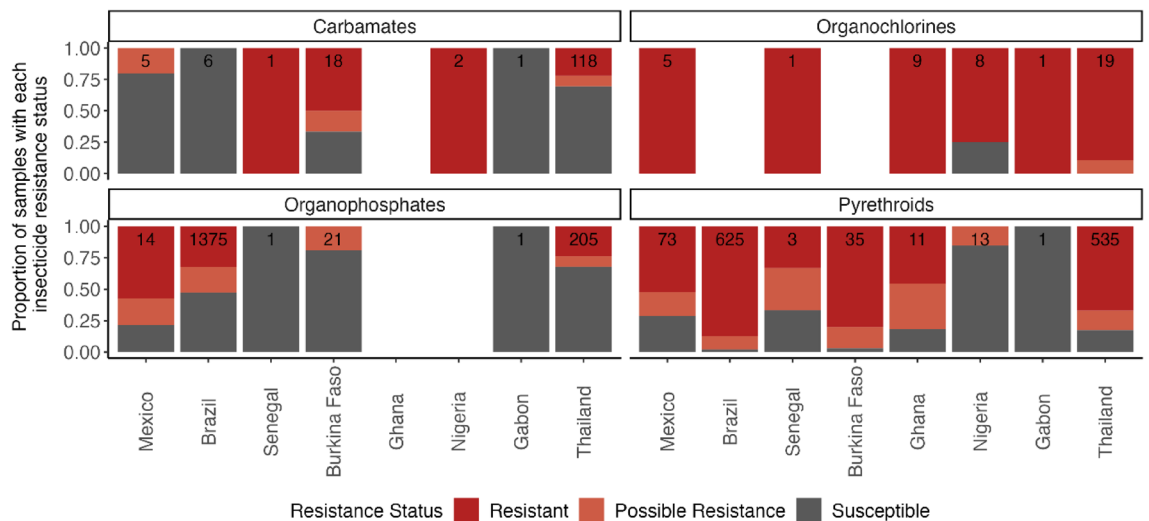
Figure 4. Publicly available phenotype data for Ae. aegypti showing the proportion of records that report resistance, possible resistance and susceptibility. Numbers denote total number of records for the insecticide class for that country region 44 . Only data collected on Aedes aegypti after 2000 were included for countries that were present in the WGS data set.
