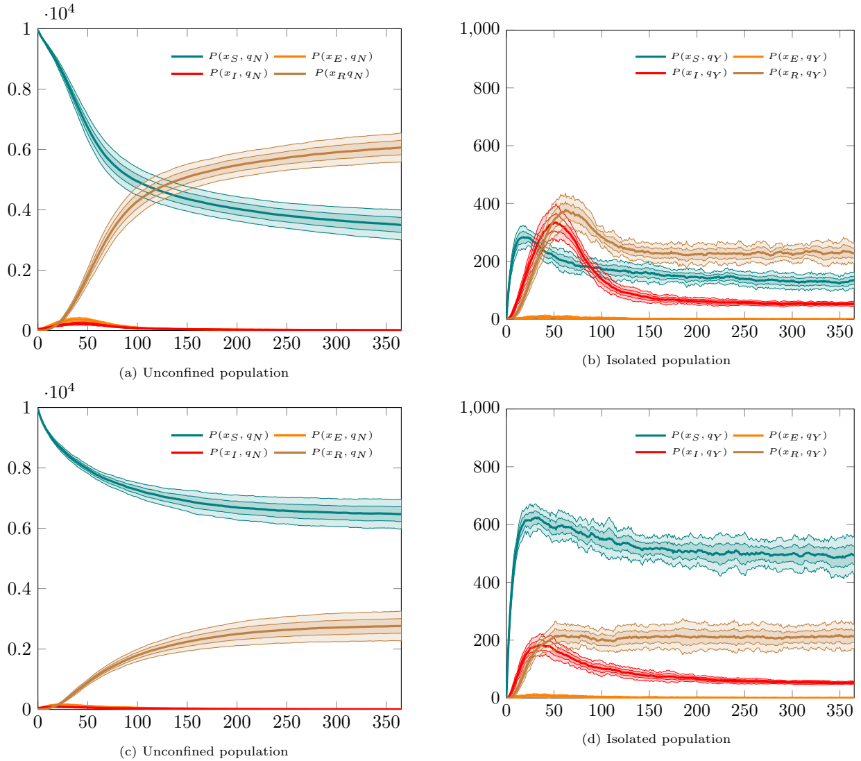
Figure 4: Resource constrained testing leading to isolation. The top row is a circumstance where sufficient tests are manufactured to test 2.5% of the population daily and the bottom row, 5%. Tests are consumed on use, and have a recall (true positives rate) and specificity (true negative rate) of 80%. A positive test leads immediately to isolation. On the left are the unconfined sub-populations and on the right are the isolated sub-populations. Infection only happens within the unconfined sub-populations.
