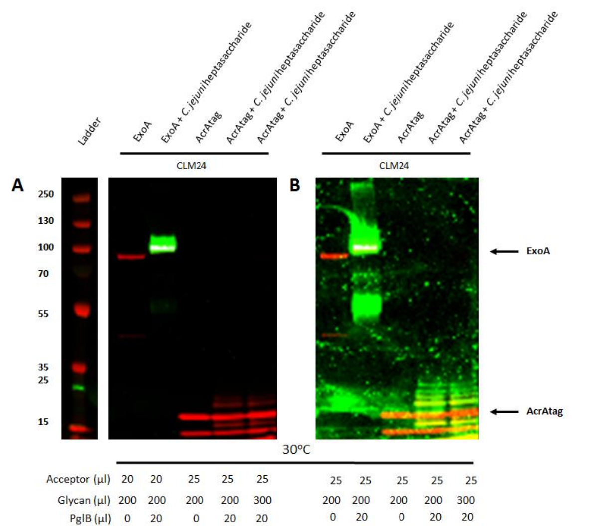
Figure 7.17. In vitro glycosylation of ExoA and AcrAtag with the C. jejuni heptasaccharide. Lysates of the C. jejuni heptasaccharide, PglB, and acceptor proteins ExoA or AcrAtag were incubated together overnight at 30°C, then the nickel affinity purified protein probed on an anti-His (red), anti-galactose (green) immunoblot. (A) standard exposure, (B) increased exposure for the green channel.
