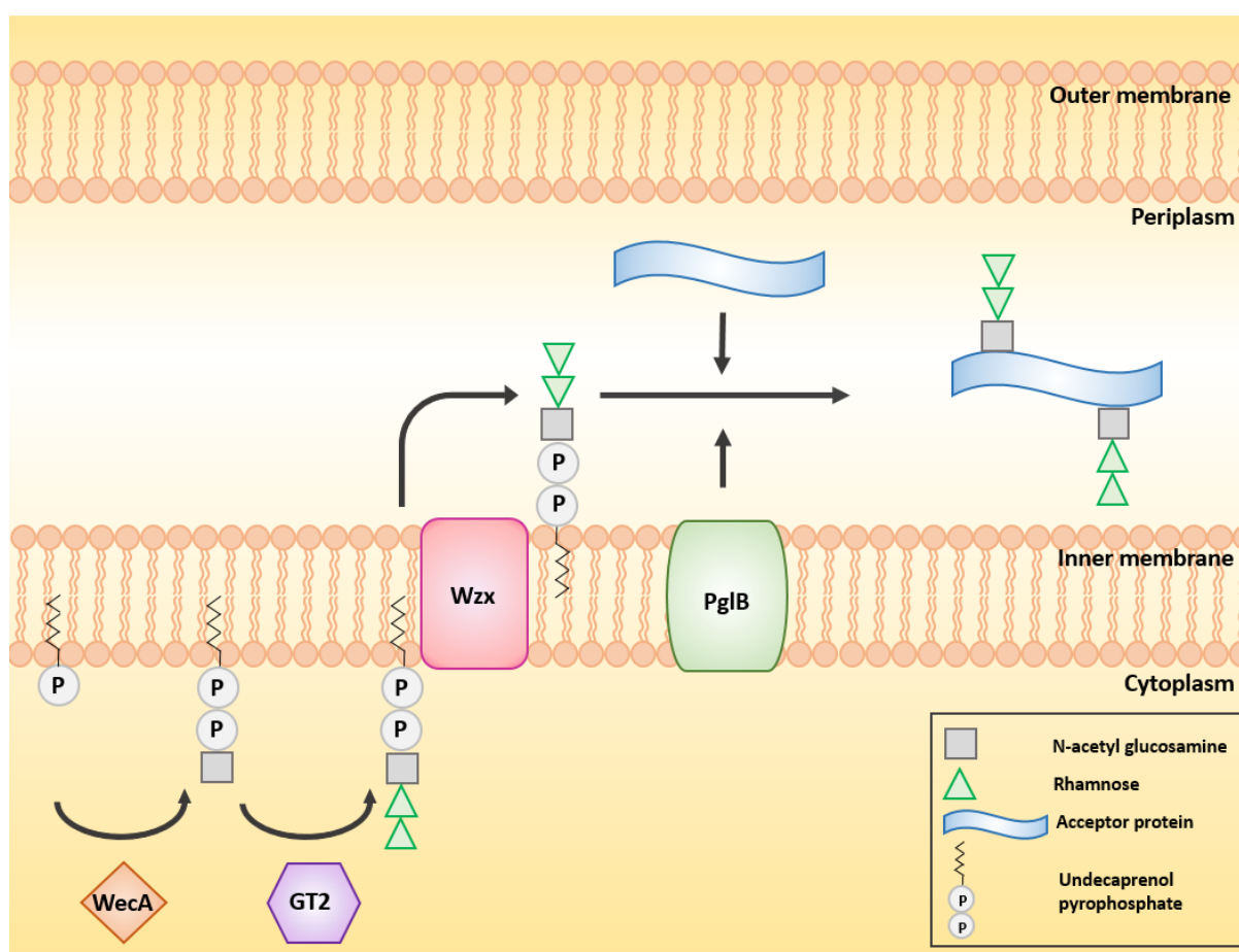
Figure 7.5. Proposed pathway for the expression of the C. difficile flagella glycan in E. coli . The E. coli enzyme, WecA, adds GlcNac onto UndPP then the C. difficile GT2 (CDR20291_0242) builds the methylated di-rhamnose structure onto this. The E. coli flippase transfers the glycan into the periplasm where it can be recognised by C. jejuni PglB and conjugated to the D-X-N-Y-S/T recognition sequon within the acceptor protein.
