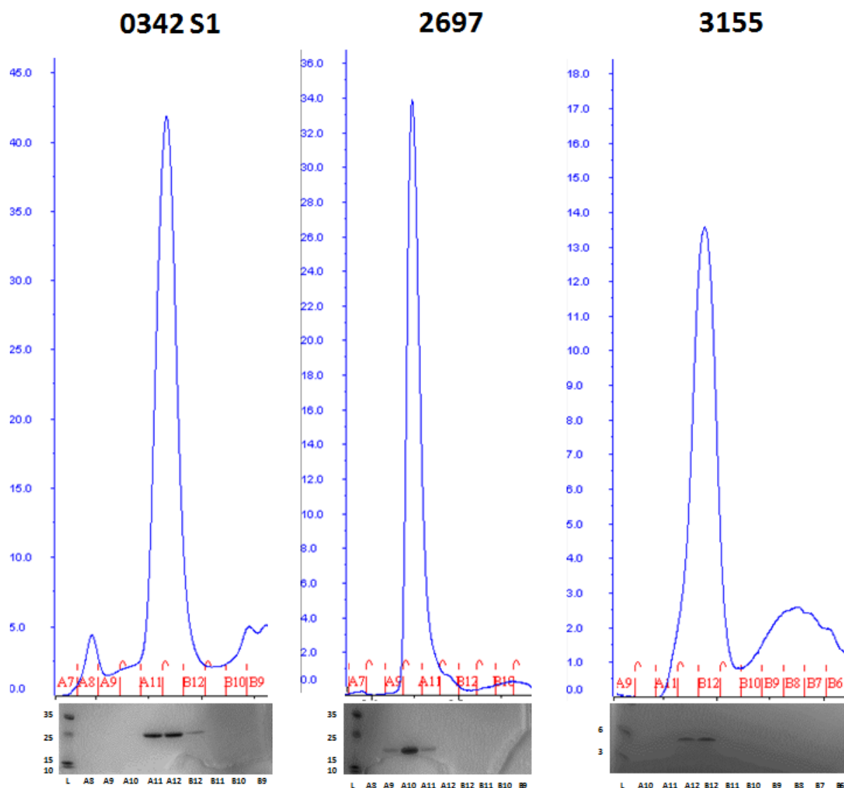
Figure 3.6. Purification of the C. difficile recombinant array candidates using gel filtration. Flow-through samples isolated from the nickel affinity purification following TEV mediated cleavage of the 6XHistag were passed through a gel filtration column as an additional purification step. This separates protein based on size and was successful for all three proteins, as demonstrated in the corresponding SDS-PAGE gels.
