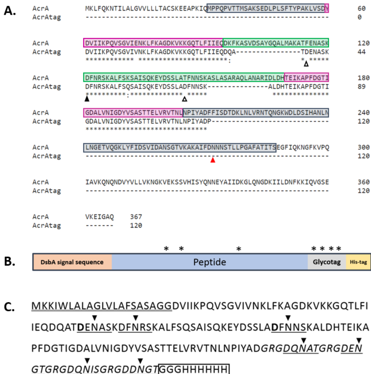
Figure 7.6. Design and sequence of the acceptor protein, AcrAtag. A short acceptor protein was designed for use in the glycosylation experiments, comprising a fragment of the C. jejuni periplasmic lipoprotein, AcrA with a four sequon glycotag. (A) Sequence alignment of full length AcrA and AcrAtag. The coloured regions represent the different protein domains; \beta barrel sandwich hybrid (grey), lipoyl domain (pink) and coiled coil domain (green) [348]. Arrows denote N -glycosylation sequons, either native (filled black), native but not used for AcrAtag (filled red) or engineered (empty). : defines residues mutated to reduce proteolytic cleavage. (B) Schematic of AcrAtag with N-terminal DsbA signal sequence for localisation to the periplasm, where PglB functions, the peptide sequence containing one native and two engineered glycosylation sequons (asterisks), the glycotag comprising four glycosylation sequons and a C-terminal 6xHis tag for nickel affinity purification. (C) Full sequence of AcrAtag; DsbA signal sequence (double underlined), N -glycosylation sequon (single underlined), glycosylated asparagine residue (arrow), mutated residue to generate another glycosylation sequon (bold), glycotag (italics), 6xHis tag (box).
