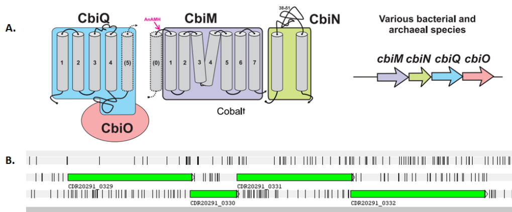
Figure 4.1. Organisation of the CbiMNQO transporter. (A) Schematic of the suggested organisation of the CbiMNQO cobalt transporter in bacteria, including the ATPase (CbiO), transmembrane components (CbiQ) and substrate binding domains (CbiM and CbiN). Image taken from Rodionov et al. [490]. (B) Genomic organisation of the putative CbiMNQO transporter in C. difficile R20291 including; CbiM (CDR20291_0329), CbiN (CDR20291_0330), CbiQ (CDR20291_0331) and CbiO (CDR20291_0332).
