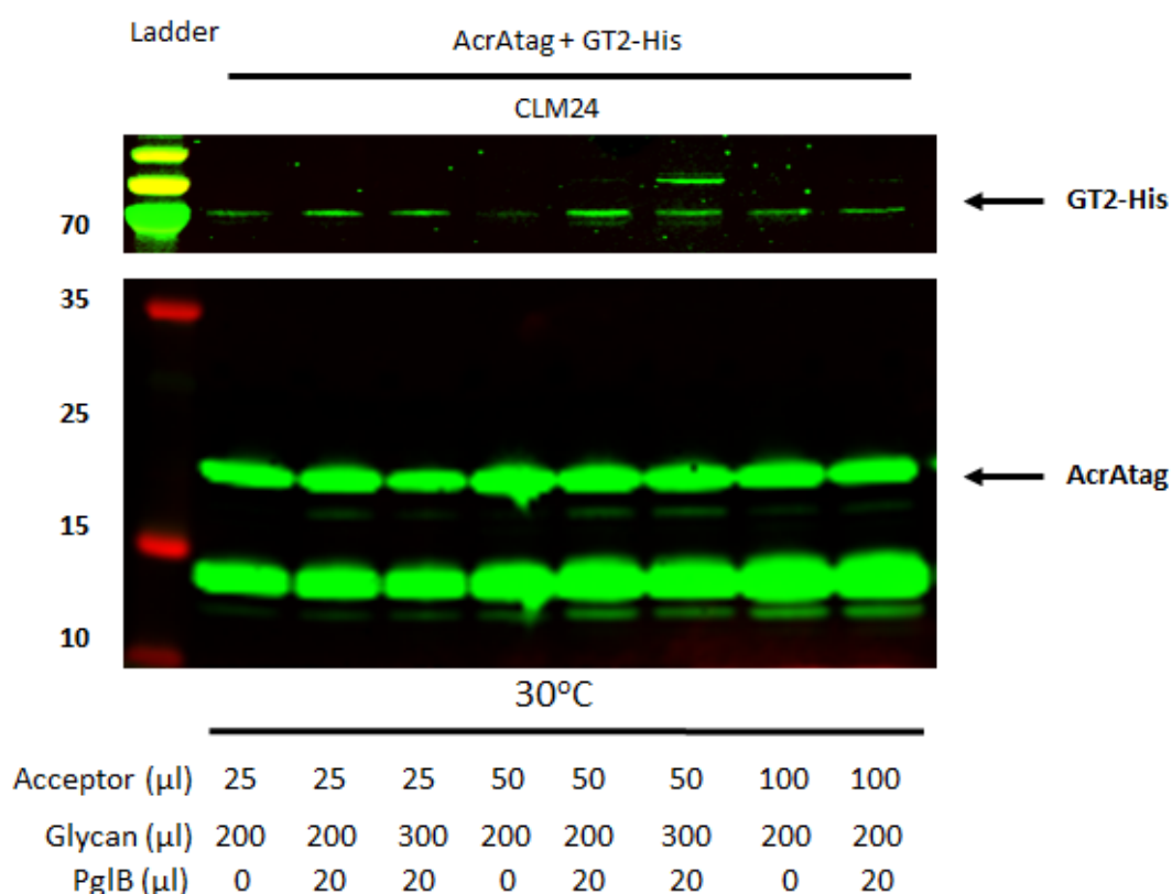
Figure 7.18. In vitro glycosylation trials of AcrAtag with the C. difficile GT2. Lysates of CLM24 harbouring GT2-His, PglB, and AcrAtag were incubated together overnight at 30°C, then the nickel affinity purified protein probed on an anti-His (green) immunoblot.
