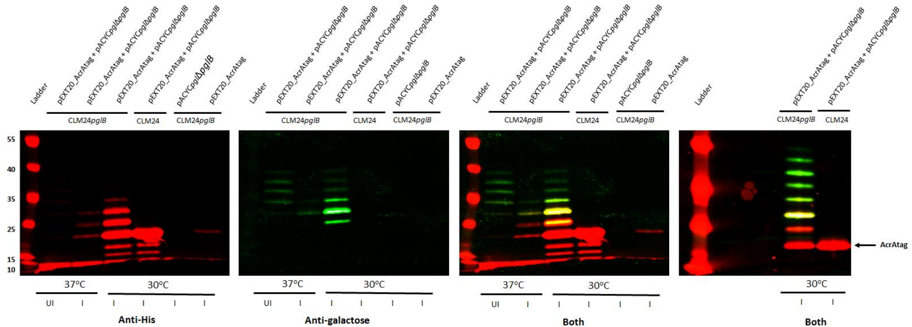
Figure 7.9. Glycosylation of IPTG-inducible AcrAtag with the C. jejuni heptasaccharide. To confirm AcrAtag could be glycosylated, the constitutive pACYCpglΔpglB construct, encoding the C. jejuni heptasaccharide locus was co-expressed with pEXT20_AcrAtag in CLM24pglB and CLM24 (no pglB) cells. These were incubated overnight at 37°C and 30°C, then induced with 1 mM IPTG: I, induced, UI, uninduced. AcrAtag was extracted and nickel affinity purified then detected by immunoblot using anti-His antibody to AcrAtag and soy bean agglutinin (SBA) lectin to the C. jejuni glycan. The first three panels present the immunoblot images with anti-His only (red), anti-glycan (anti-galactose) only (green) then the two overlaid. The last panel displays a repeat expression test.
