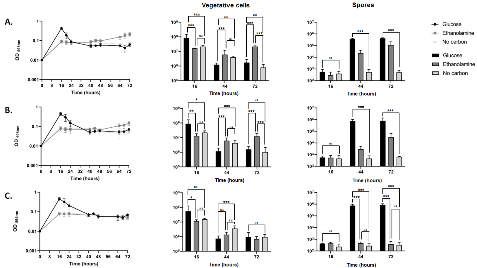
Figure 4.10. Growth kinetics of 630Δerm, 630Δerm_1910::CT and 630Δerm_1911::CT in ethanolamine. Strains were grown to OD 0.6 in rich media before inoculation into minimal media containing glucose, ethanolamine or water (no carbon control). OD 595 readings were taken at 16, 20, 24, 40, 44, 48, 64, 68 and 72 hours. Colony forming units for the total cell and spore counts were also taken at 16, 44 and 72 hours. Spore counts were incubated at 65°C for 20 mins before plating to remove vegetative cells then vegetative cell count was calculated by subtracting the spore count from the total cell count. (A) 630Δerm, (B) 630Δerm_1910::CT and (C) 630Δerm_1911::CT. Differences in CFU counts between strains was analysed for significance using a linear regression. * p > 0.05 , p > 0.005 , p > 0.0005 , NS- not significant. Each culture was set up in duplicate and three independent replicates were performed. Error bars represent standard deviation.
