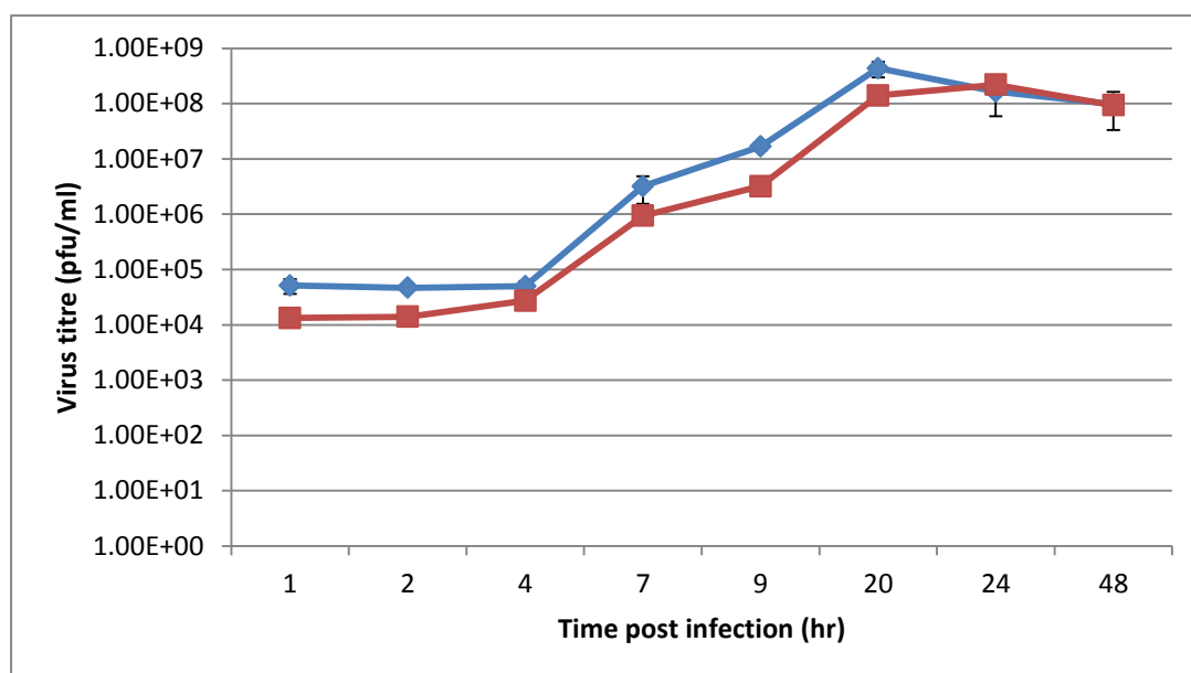
Figure 3.4 Growth curves of wild type (wt) and A533V mutant (mut) viruses (blue and red respectively). Vero cells were infected at a multiplicity of infection (MOI) of 0.01pfu with CHIK-SL(r-wt) and CHIK-SL(r-mut). Cell culture supernatants were harvested at the indicated times and viral progeny titres determined by plaque assays in triplicate. Each data point represents the mean average of the virus titre and the error bars denote standard deviation.
