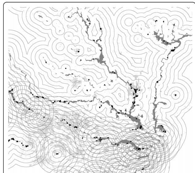
Figure 2 GIS generated 'map' of a local area illustrating the definition of boundaries of 0-, 2-, 4-, 6-, and 8-10 km (gray lines) around flood areas (dark gray filled boundaries).
