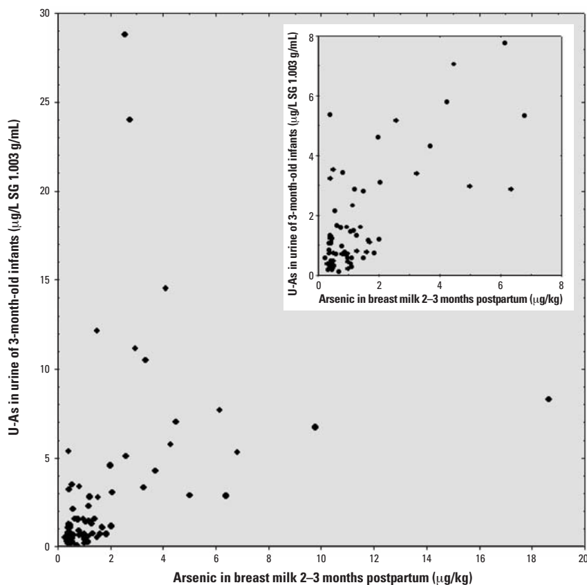
Figure 2. Scatterplot between the sum of arsenic metabolites (iAs, MA, and DMA) in urine ( \mu\text{g}/\text{L} , SG 1.003 g/mL) of 3-month-old infants and the concentrations of arsenic in breast milk ( \mu\text{g}/\text{kg} ) ( r_s = 0.64 , p < 0.001 , n = 79 ). Inset shows an enlargement of the diagram at the low concentration range.
