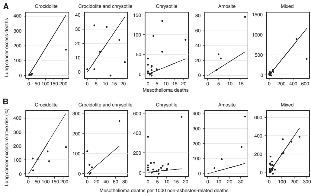
Figure 1 (A) Ratio 1 components, absolute excess lung cancer excess deaths vs mesothelioma deaths, by asbestos type. (B) Ratio 2 components, lung cancer excess relative risk (%) vs mesothelioma deaths per 1000 non-asbestos-related deaths, by asbestos type. Note that graphs are not to the same scale. The reference line on each sub-graph corresponds to the same ratio estimate (average values for mixed fibres from Table 3); thus, the distribution of points about this line can be compared across subgraphs.
