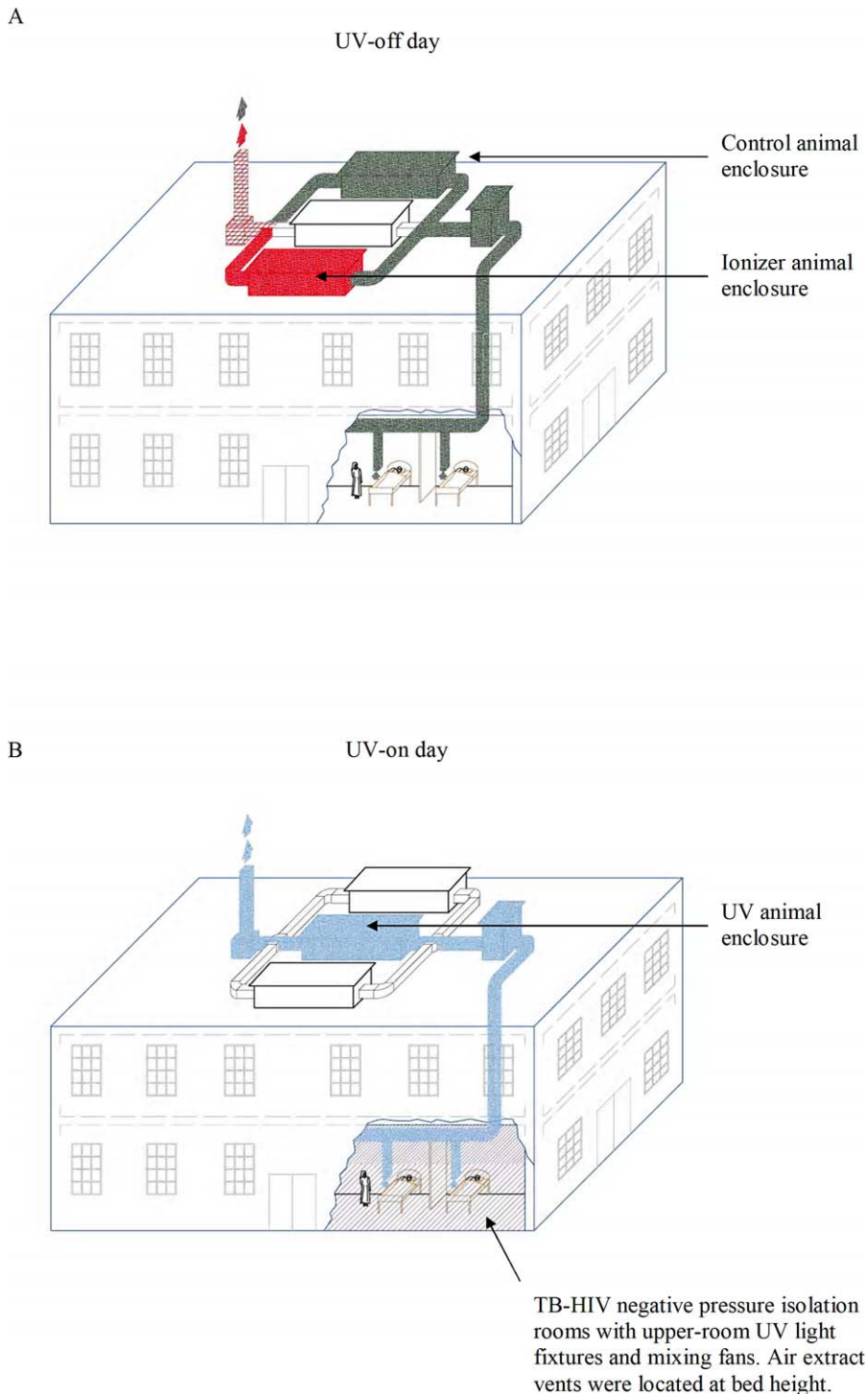
Figure 2. Schematic of the Airborne TB Transmission Study Facility on the Roof of an HIV-TB Ward in Lima, Perú
