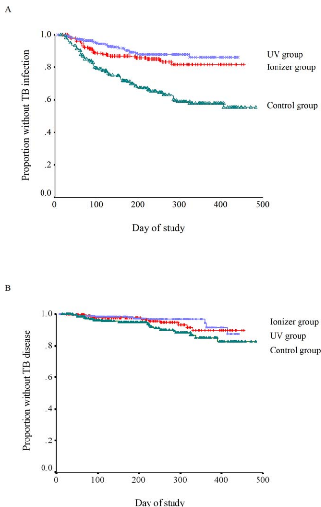
Figure 6. Kaplan-Meier Time-to-Event Curves
