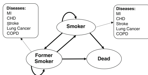
Fig. 1 Markov model
