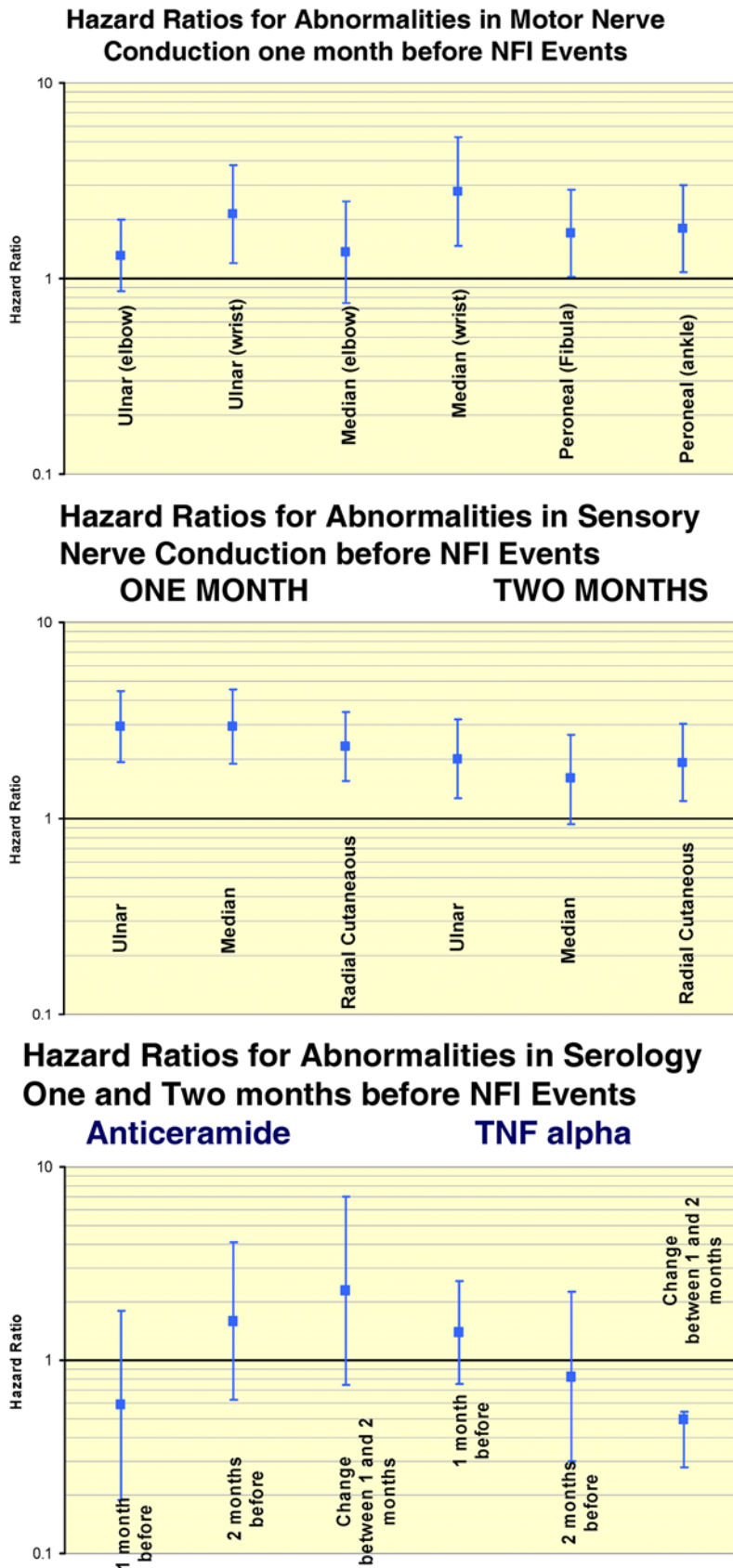
Figure 3. Adjusted hazard ratios for new nerve function impairment events for motor and sensory conduction, and serology abnormalities before an event.
